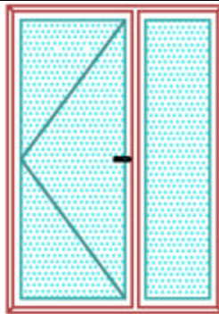
Main Entrance DOOR with side lite Min. size: w 5' x h 6.5' Max. size: w 7.5' x h 8'
