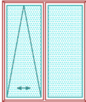
Tilt & Slide DOOR Min. size: w 8' x h 6.5' Max. size: w 13' x h 8.5'
