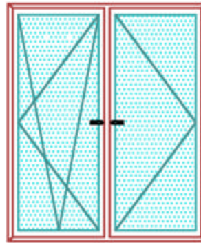
Double Balcony DOOR Min. size: w 4.5' x h 6.5' Max. size: w 7.5' x h 8'
