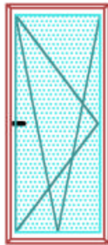
Tilt & Turn Balcony DOOR Min. size: w 2.5' x h 6.5' Max. size: w 4.2' x h 8'
