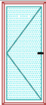
Main Entrance DOOR Min. size: w 2.5' x h 6.5' Max. size: w 4.2' x h 8'
