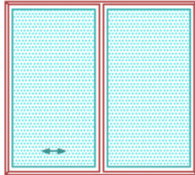
Large Lift & Slide DOOR Min. size: w 13.5' x h 6.5' Max. size: w 18.5' x h 8.5'
